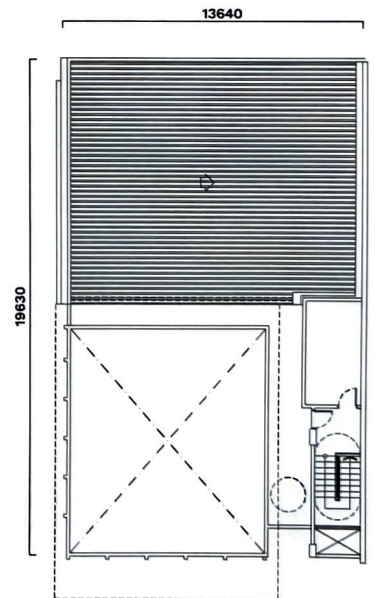
ROOF FLOOR
